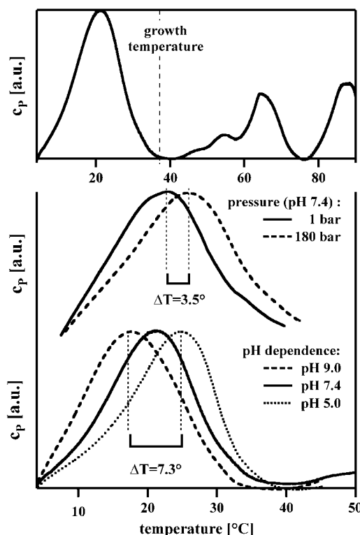
FIGURE 2 Heat capacity profiles of native E. coli membranes. (Top) At 37°C. The growth temperature is indicated. The large peak below growth temperature corresponds to lipid melting. The smaller peaks above growth temperature correspond to protein unfolding. (Center) The heat capacity as a function of T at a hydrostatic pressure of 1 bar and 180 bar. The pressure-induced shift is \approx 3.5 K. (Bottom) Heat capacities for the same membranes at various pH values. The transition temperature increases by \sim 5.3 K when the pH is reduced from 7.4 to 5.0. Scans were halted at 40–43°C to prevent protein unfolding.
