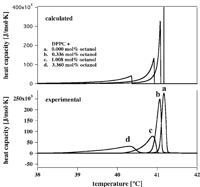
FIGURE 1 The effect of octanol on the phase transition of DPPC vesicles. (Bottom) Calorimetric data with various octanol concentrations in the membrane. (Top) Calorimetric profiles calculated for the same membrane concentrations of a solute assuming ideal mixing in the fluid phase and no mixing in the gel phase. The high temperature end of the transition profile corresponds to the temperature calculated for melting point depression. The calculation assumes a finite bulk fluid phase. This leads to an accumulation of anesthetics in the fluid phase as the temperature is lowered and to an asymmetric broadening of the c_p profile.
